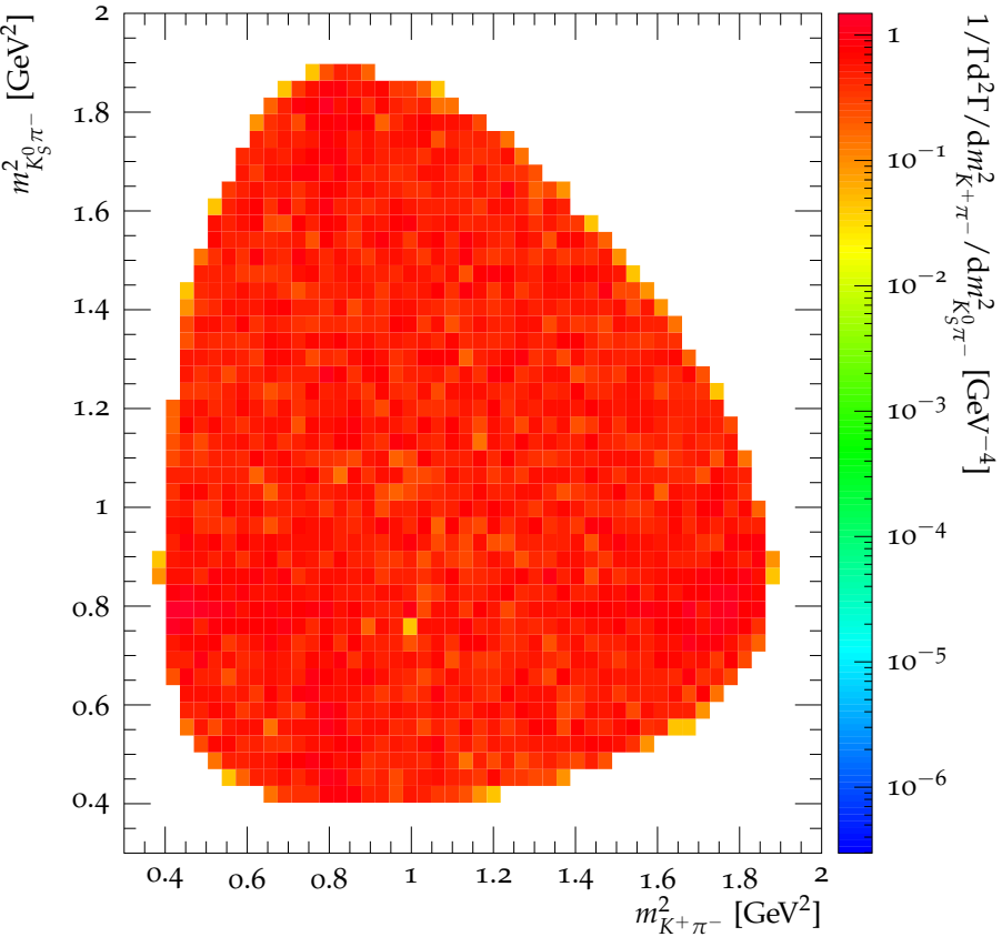
Dalitz plot for D^0 \rightarrow K_S^0 K^+ \pi^-
