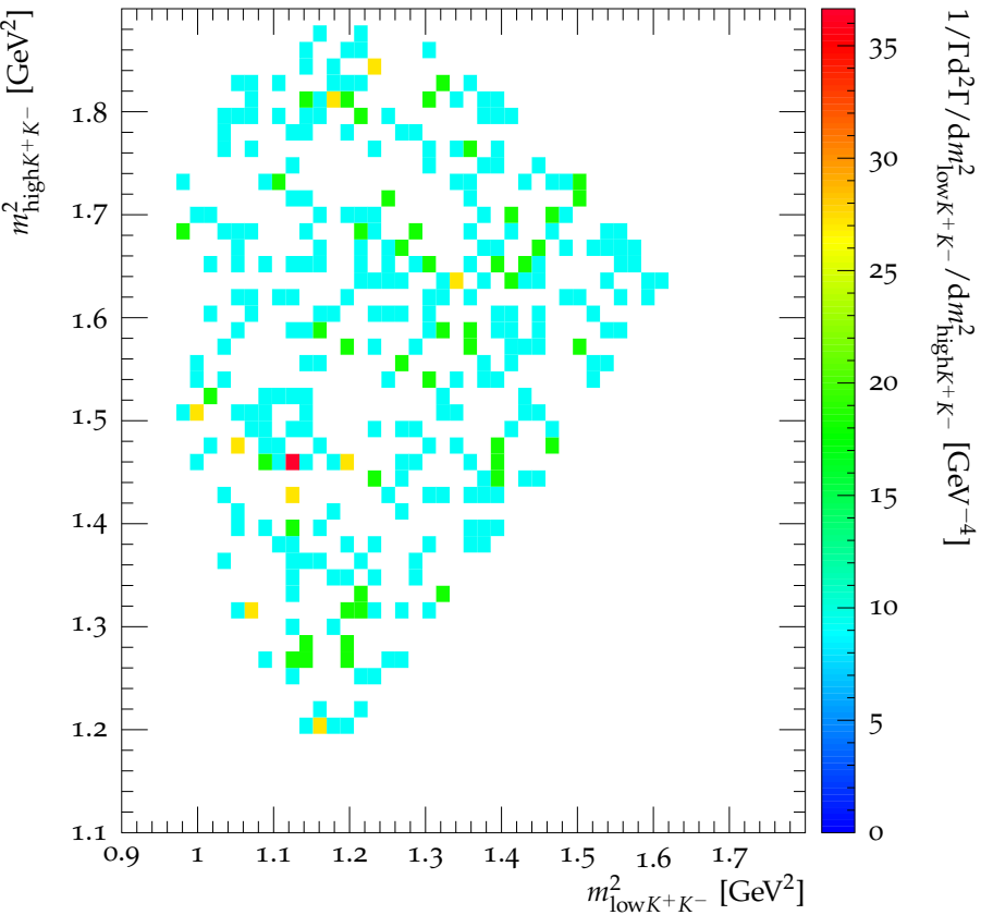
Dalitz plot for D^+ \rightarrow K^+K^+K^-
