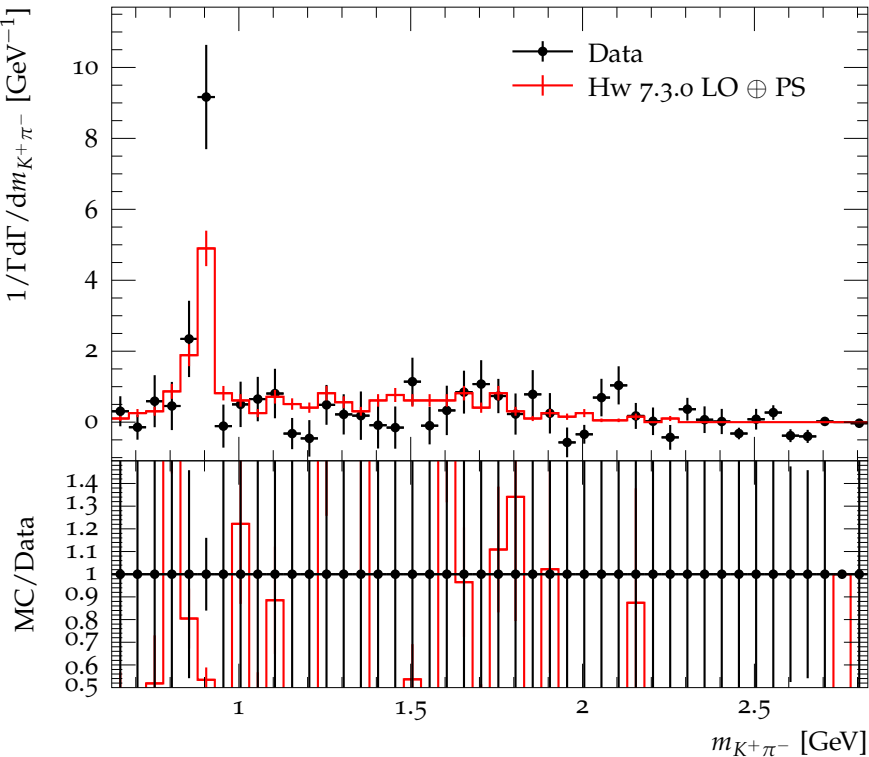
K^+ \pi^- mass distribution in B_c^+ \rightarrow J/\psi K^+ \pi^- \pi^+
