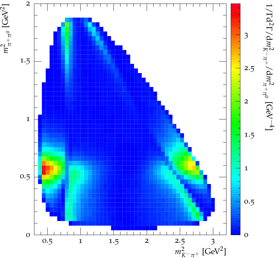
Dalitz plot for D^0 \rightarrow K^- \pi^+ \pi^0
