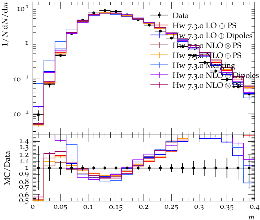
Thrust minor, m (charged+neutral) (average)
