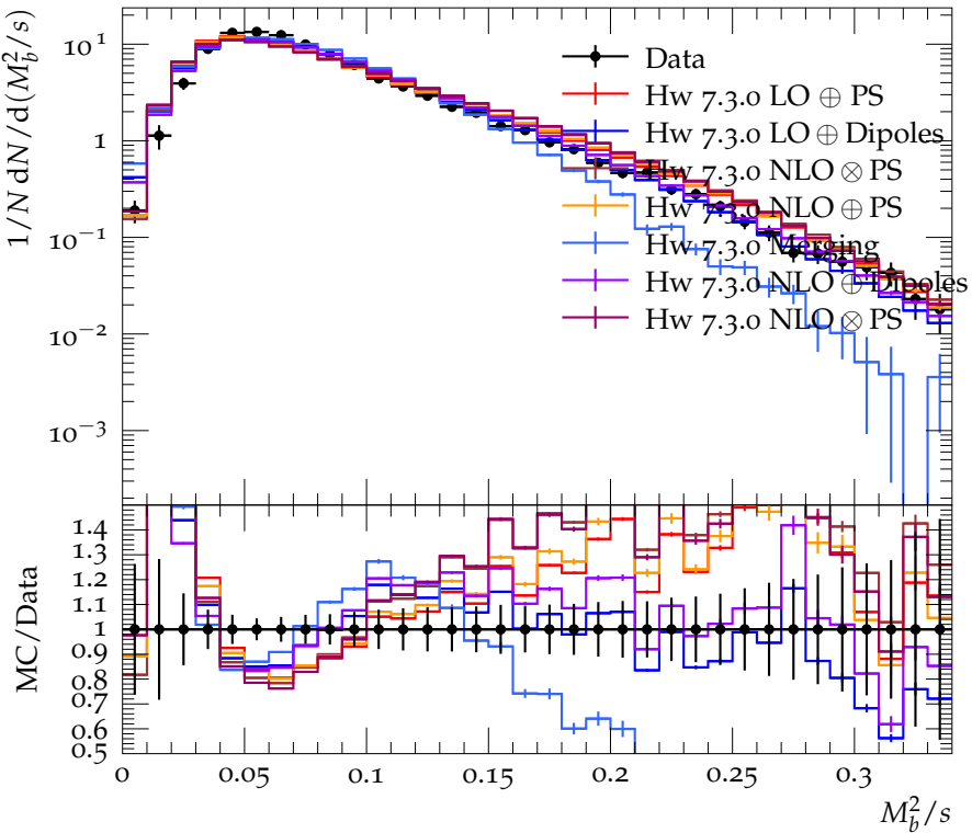
Broad jet mass (charged+neutral) (average)
