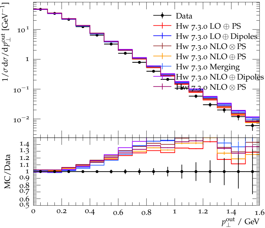
Out-plane p_T out GeV w.r.t. sphericity axes (charged) (average)
