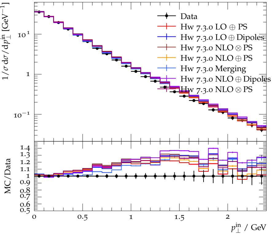
In-plane p_T in GeV w.r.t. sphericity axes (charged) (average)
