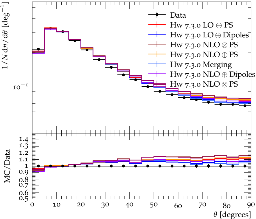
Charged particle flow w.r.t. rapidity axes (charged) (average)
