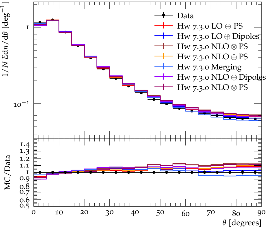
Energy flow w.r.t. rapidity axes (charged+neutral) (average)
