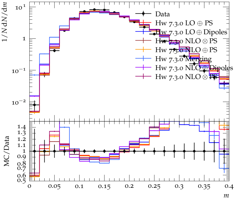
Thrust minor, m (charged+neutral) (PEP5)
