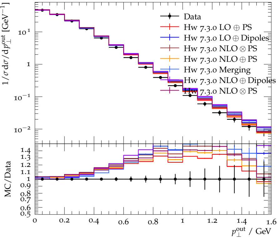
Out-plane p_T out GeV w.r.t. sphericity axes (charged) (PEP5)
