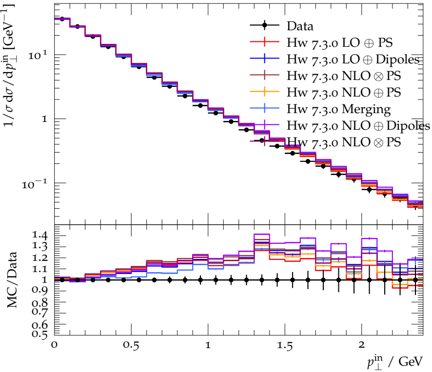
In-plane p_T in GeV w.r.t. sphericity axes (charged) (PEP5)
