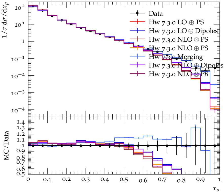
Scaled momentum, x_p = |p|/|p_{\text{beam}}| (charged) (PEP5)
