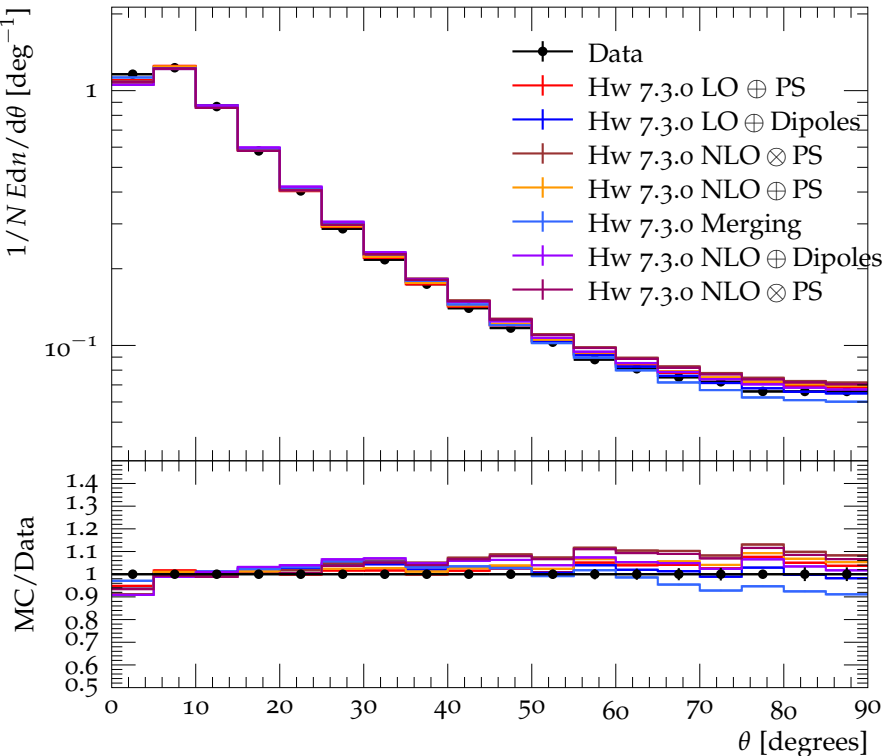
Energy flow w.r.t. rapidity axes (charged+neutral) (PEP5)
