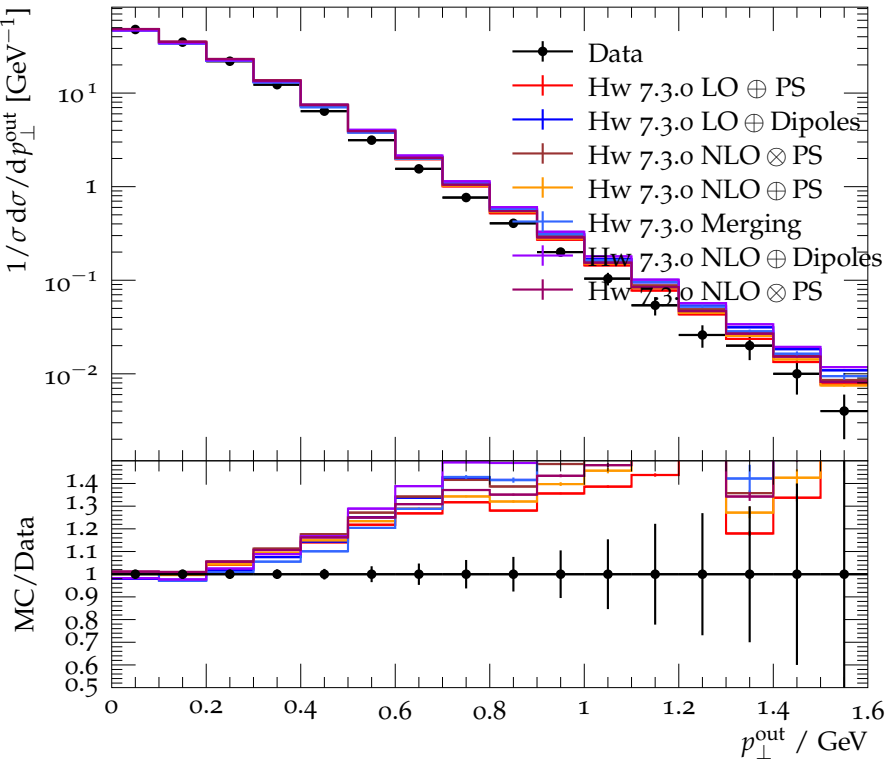
Out-plane p_T out GeV w.r.t. sphericity axes (charged) (upgrade)
