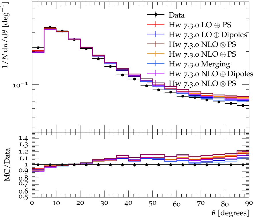
Charged particle flow w.r.t. rapidity axes (charged) (upgrade)
