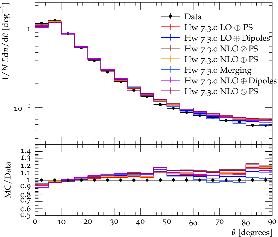
Energy flow w.r.t. rapidity axes (charged+neutral) (upgrade)
