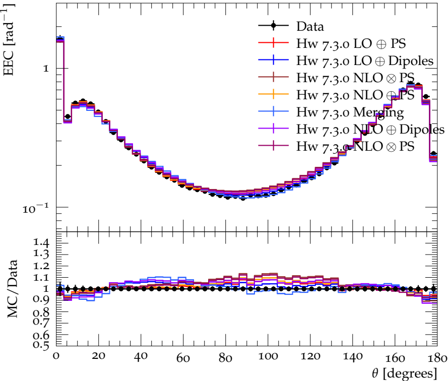
Energy-energy correlation with E_{\text{CMS}} = 29 \text{ GeV} (PEP5)
