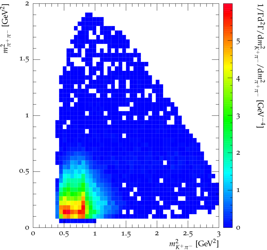
Dalitz plot for D^+ \rightarrow K^+ \pi^- \pi^+
