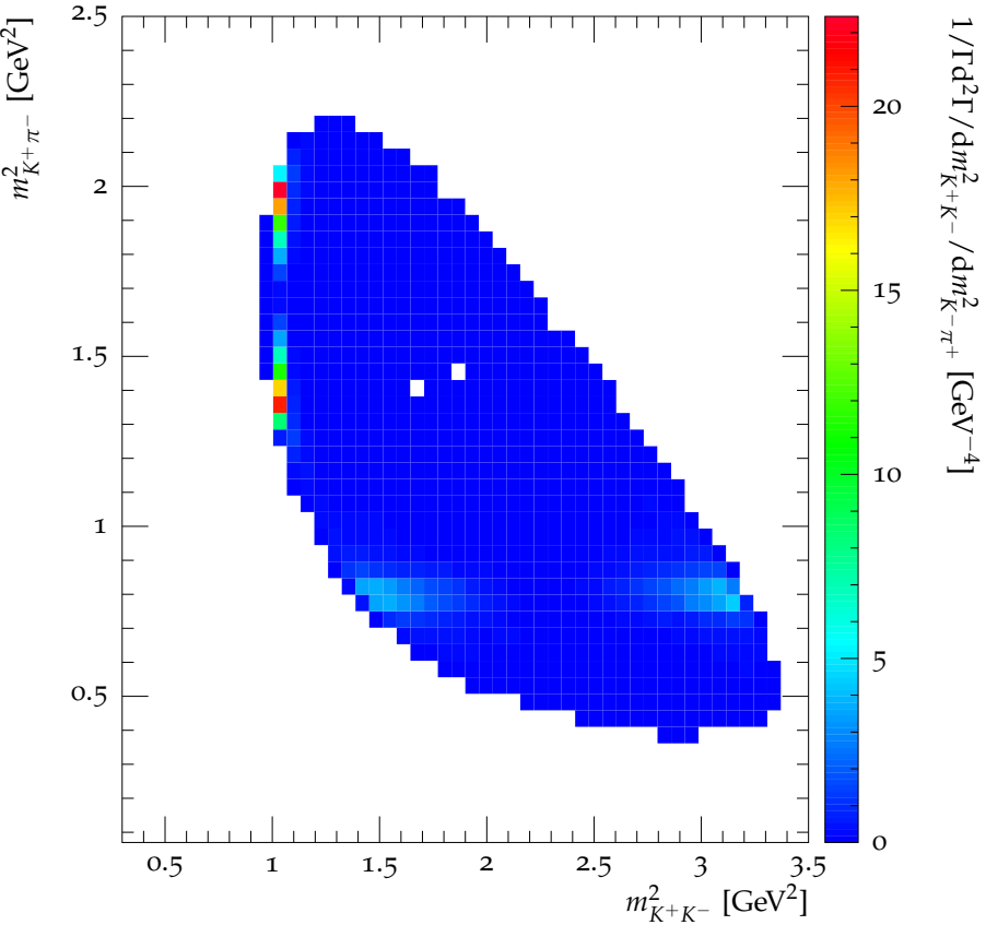
Dalitz plot for D_s^+ \rightarrow K^+K^-\pi^+
