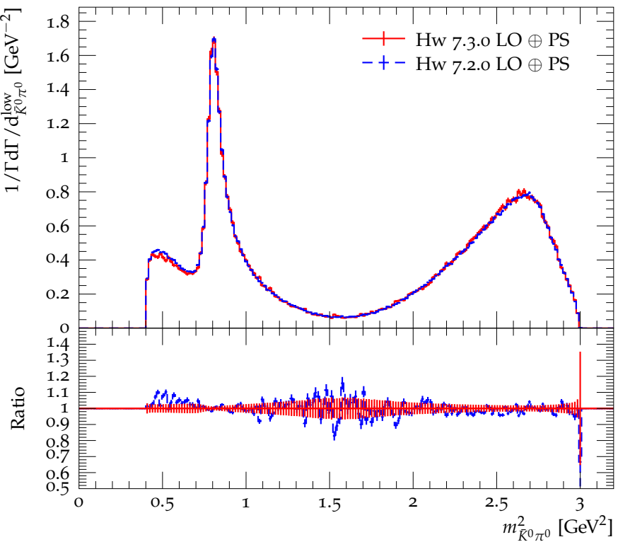
\bar{K}^0\pi^0 mass distribution in D^+ \rightarrow \bar{K}^0\pi^+\pi^0
