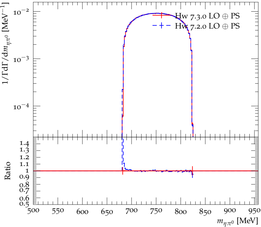
Distribution of the \eta\pi^0 mass in the decay \eta' \rightarrow \eta\pi^0\pi^0
