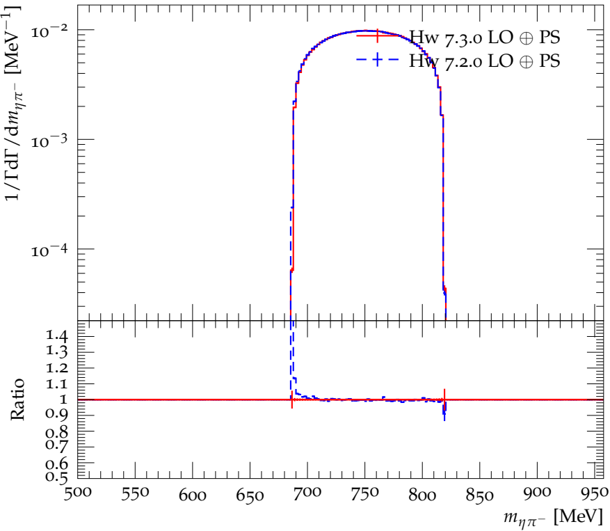
Distribution of the \eta\pi^- mass in the decay \eta' \rightarrow \eta\pi^+\pi^-
