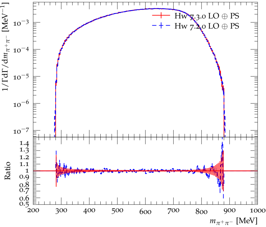
\pi^+\pi^- mass distribution in \phi \rightarrow \pi^0\pi^+\pi^- decays
