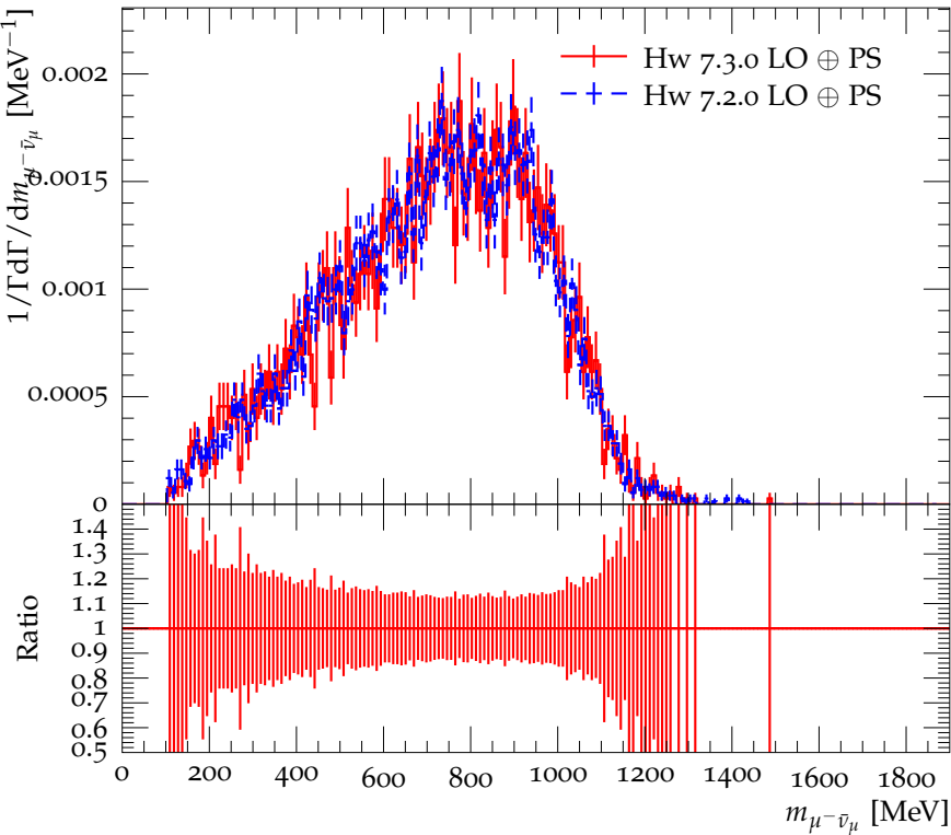
Mass of \mu^- \bar{\nu}_\mu in the decay D^- \rightarrow \rho^0 \mu^- \bar{\nu}_\mu
