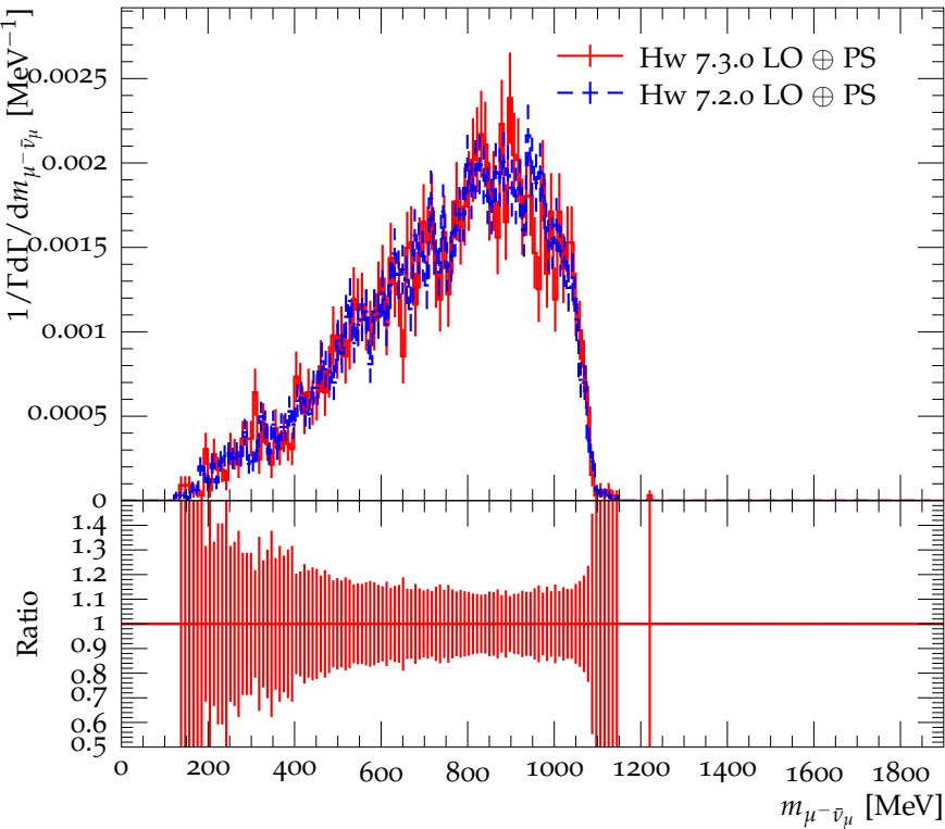
Mass of \mu^- \bar{\nu}_\mu in the decay D^- \rightarrow \omega \mu^- \bar{\nu}_\mu
