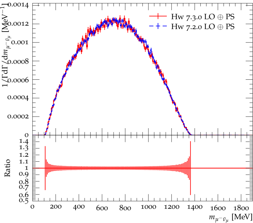
Mass of \mu^- \bar{\nu}_\mu in the decay D^- \rightarrow K^0 \mu^- \bar{\nu}_\mu
