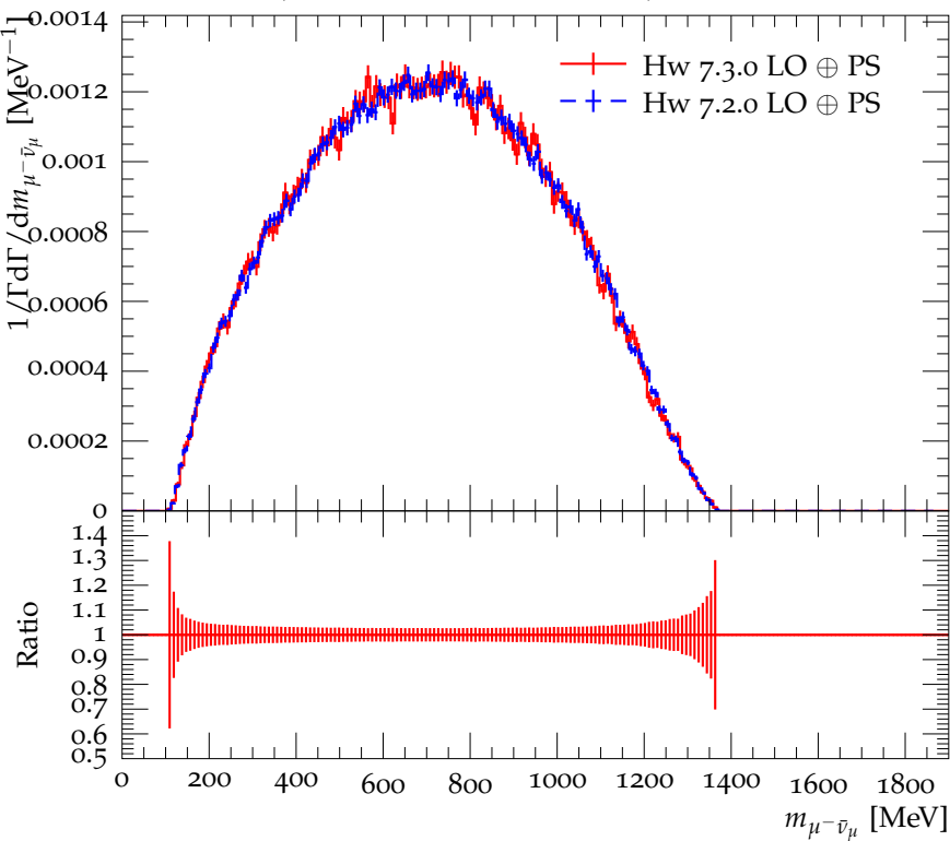
Mass of \mu^- \bar{\nu}_\mu in the decay D^0 \rightarrow K^+ \mu^- \bar{\nu}_\mu
