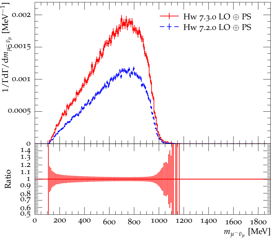
Mass of \mu^- \bar{\nu}_\mu in the decay D^0 \rightarrow K^{*+} \mu^- \bar{\nu}_\mu
