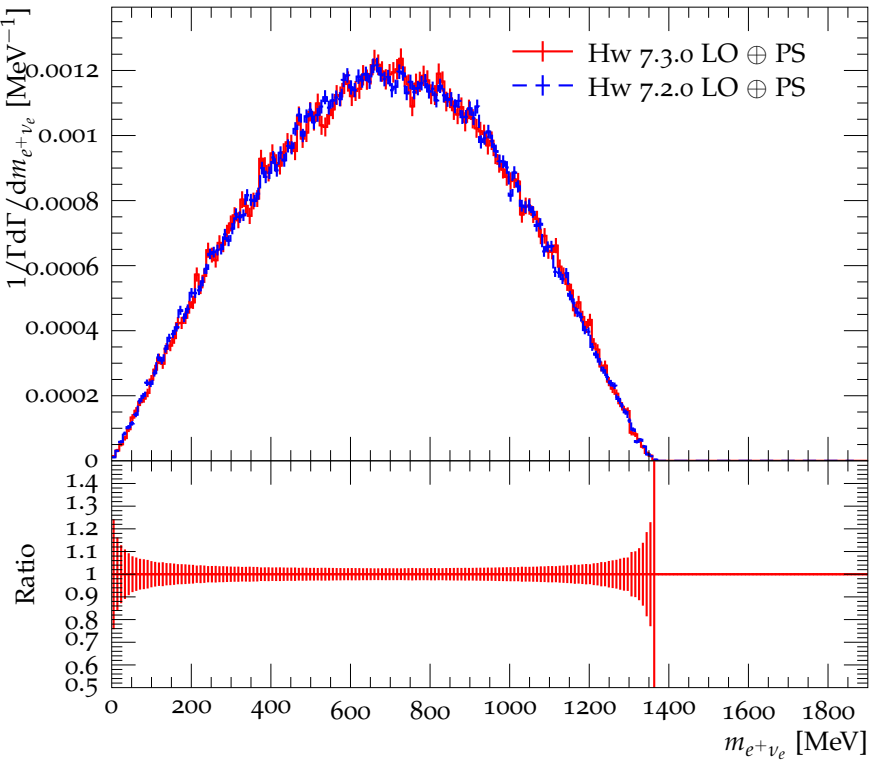
Mass of e^+ \nu_e in the decay \bar{D}^0 \rightarrow K^- e^+ \nu_e
