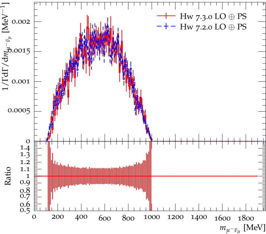
Mass of \mu^- \bar{\nu}_\mu in the decay D_s^- \rightarrow \eta' \mu^- \bar{\nu}_\mu
