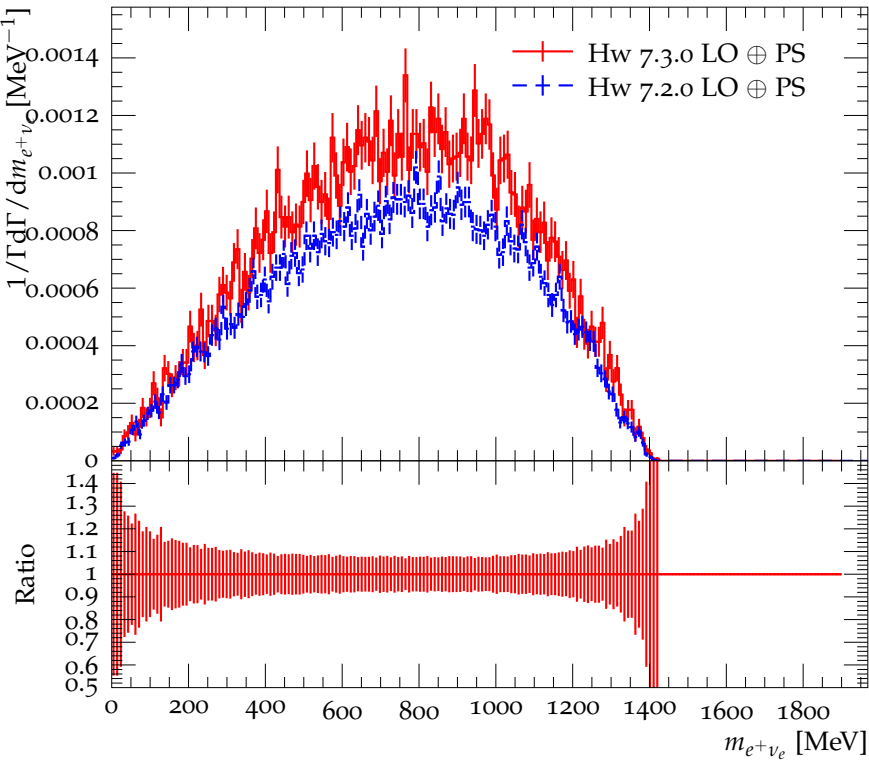
Mass of e^+v_e in the decay D_s^+ \rightarrow \eta e^+ v_e
