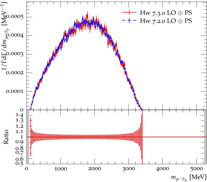
Mass of \mu^- \bar{\nu}_\mu in the decay \bar{B}^0 \rightarrow D^+ \mu^- \bar{\nu}_\mu
