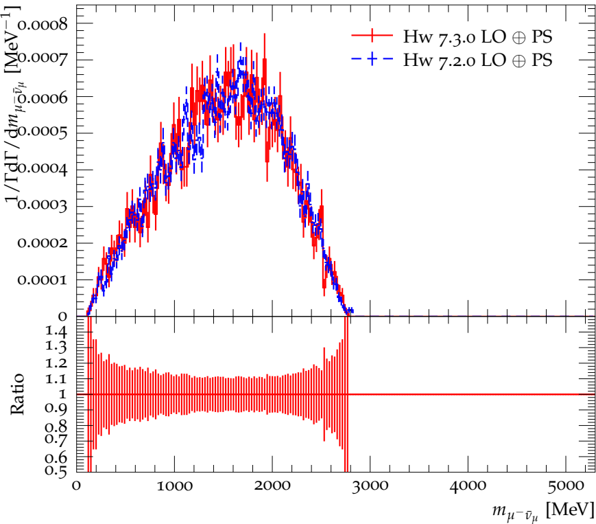
Mass of \mu^- \bar{\nu}_\mu in the decay \bar{B}^0 \rightarrow D_2^+ \mu^- \bar{\nu}_\mu
