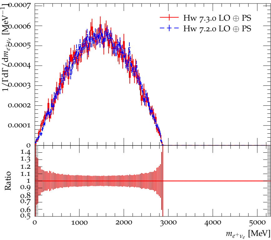
Mass of e^+ \nu_e in the decay B^0 \rightarrow D_1(2420)^- e^+ \nu_e
