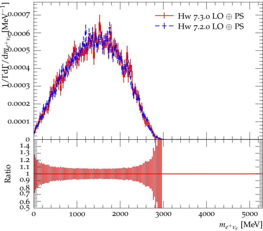
Mass of e^+ \nu_e in the decay B^0 \rightarrow D_1(2430)^- e^+ \nu_e
