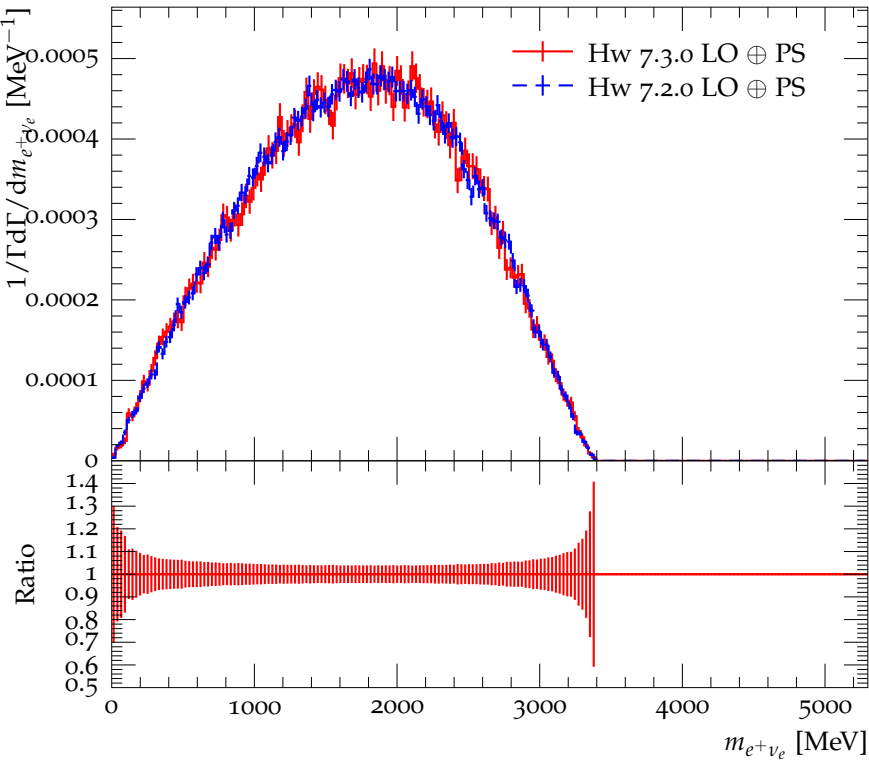
Mass of e^+ \nu_e in the decay B^0 \rightarrow D^- e^+ \nu_e
