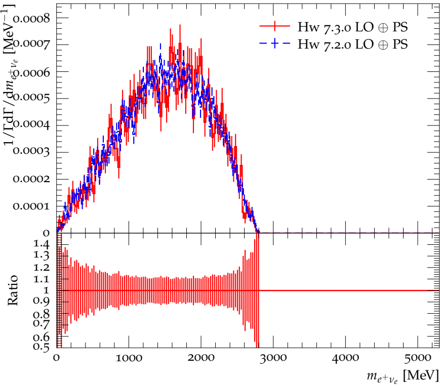
Mass of e^+ \nu_e in the decay B^0 \rightarrow D_2^- e^+ \nu_e
