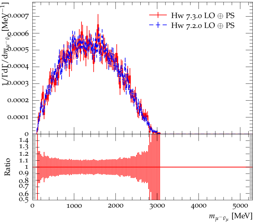
Mass of \mu^- \bar{\nu}_\mu in the decay B^- \rightarrow D_0^*(2400)^0 \mu^- \bar{\nu}_\mu
