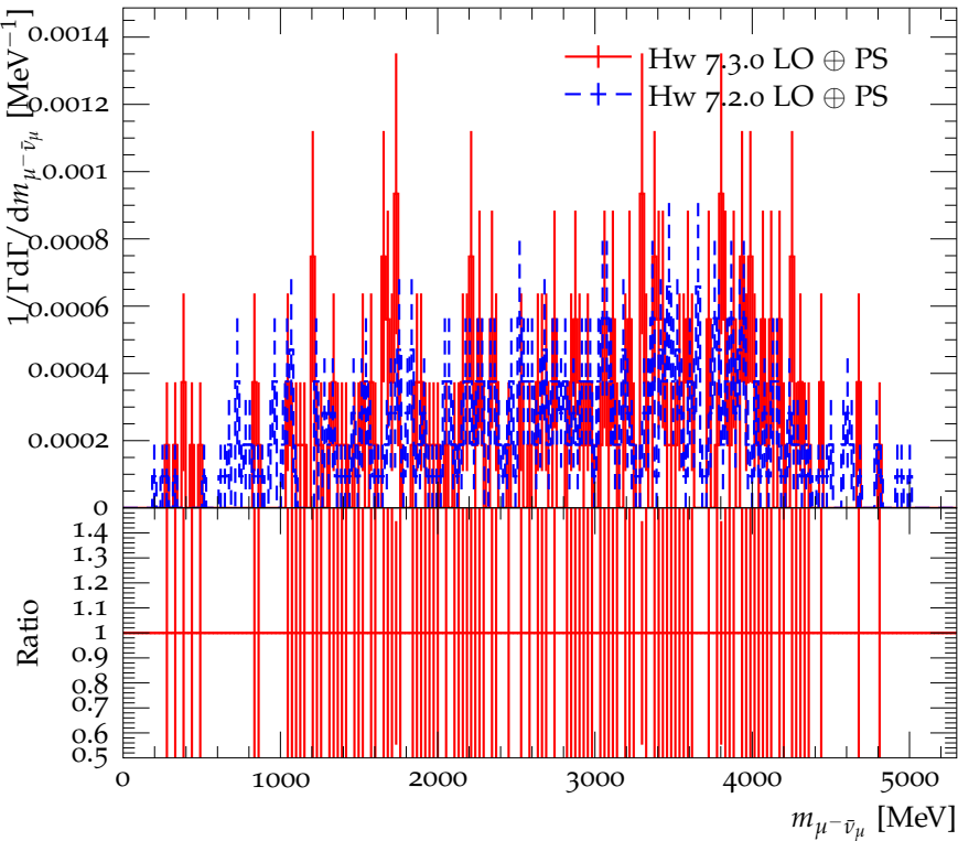
Mass of \mu^- \bar{\nu}_\mu in the decay B^- \rightarrow \pi^0 \mu^- \bar{\nu}_\mu
