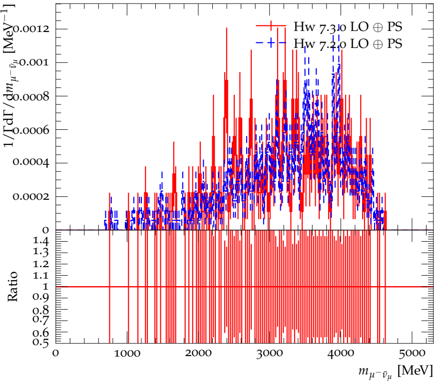
Mass of \mu^- \bar{\nu}_\mu in the decay B^- \rightarrow \rho^0 \mu^- \bar{\nu}_\mu
