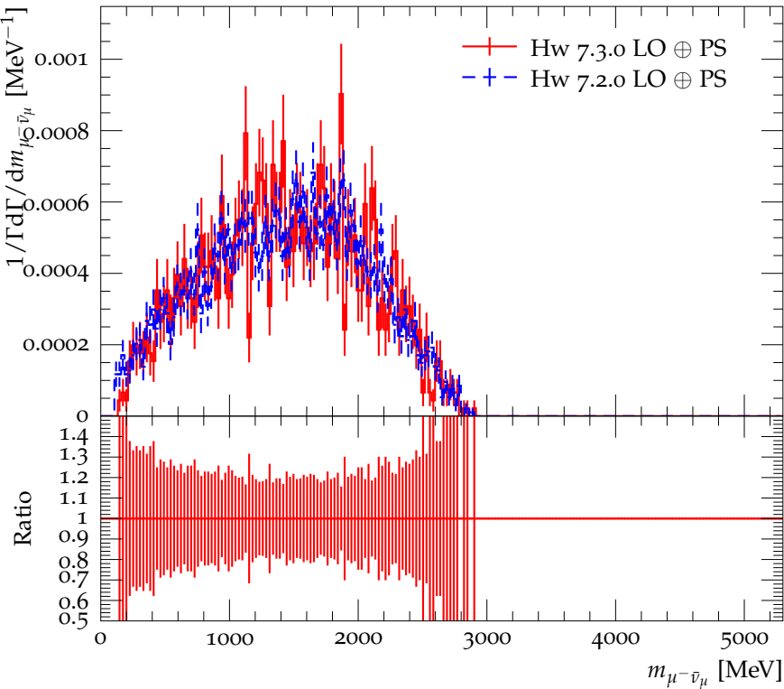
Mass of \mu^- \bar{\nu}_\mu in the decay B^- \rightarrow D_1(2430)^0 \mu^- \bar{\nu}_\mu
