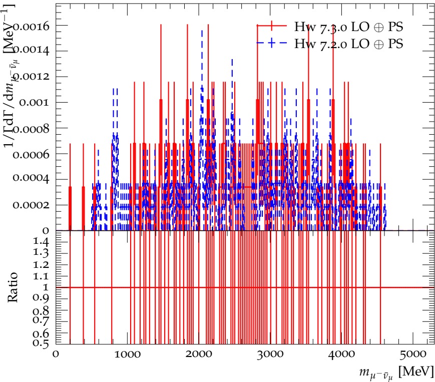
Mass of \mu^- \bar{\nu}_\mu in the decay B^- \rightarrow \eta \mu^- \bar{\nu}_\mu
