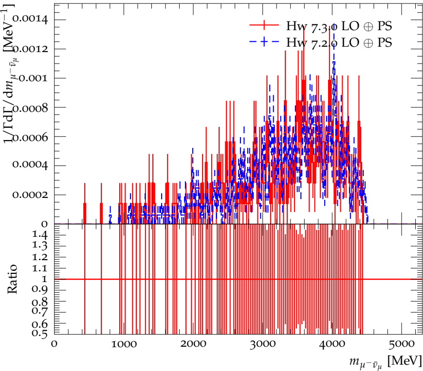
Mass of \mu^- \bar{\nu}_\mu in the decay B^- \rightarrow \omega \mu^- \bar{\nu}_\mu
