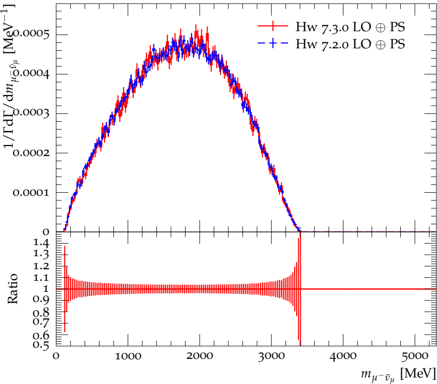
Mass of \mu^- \bar{\nu}_\mu in the decay B^- \rightarrow D^0 \mu^- \bar{\nu}_\mu
