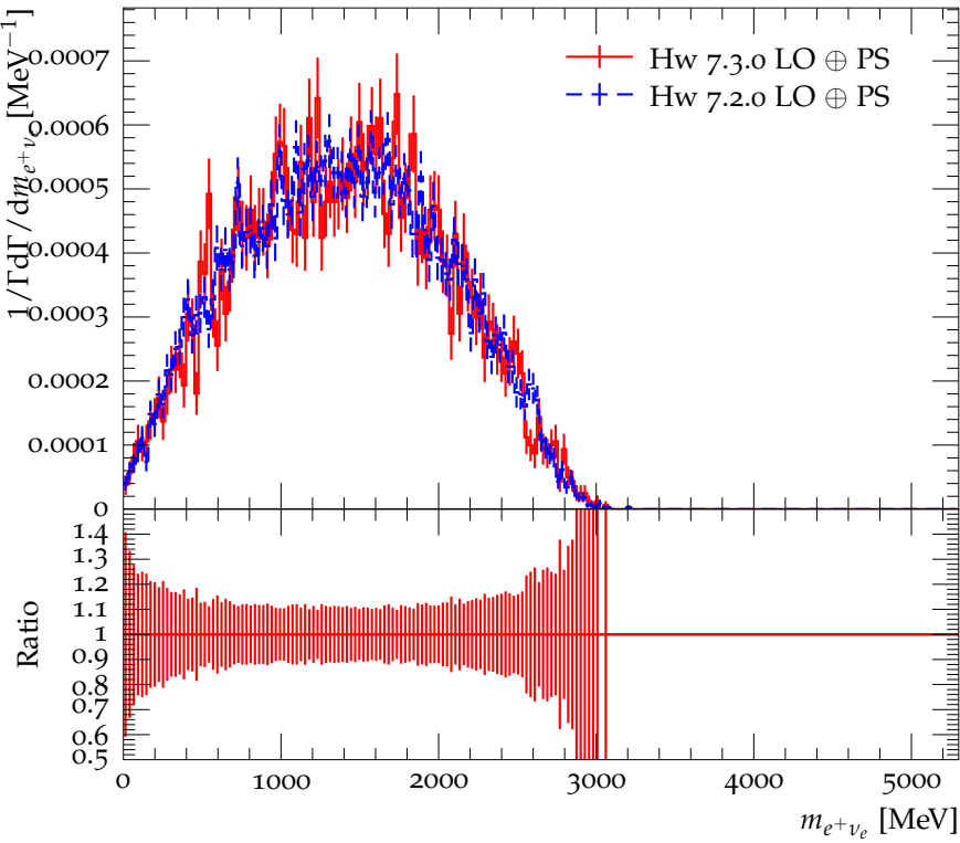
Mass of e^+ \nu_e in the decay B^+ \rightarrow \bar{D}_0^*(2400)^0 e^+ \nu_e
