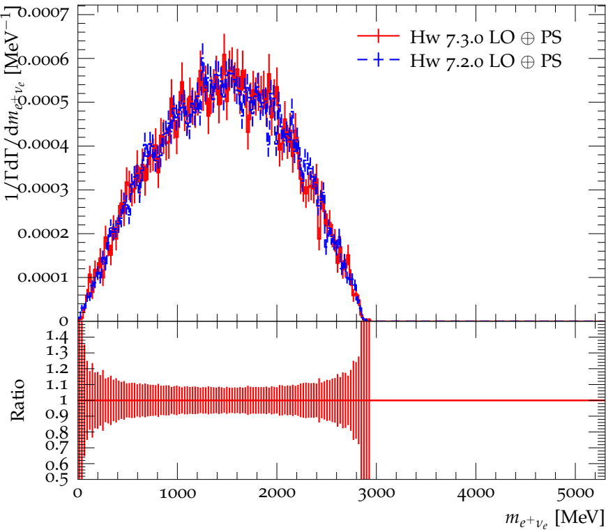
Mass of e^+ \nu_e in the decay B^+ \rightarrow \bar{D}_1(2420)^0 e^+ \nu_e
