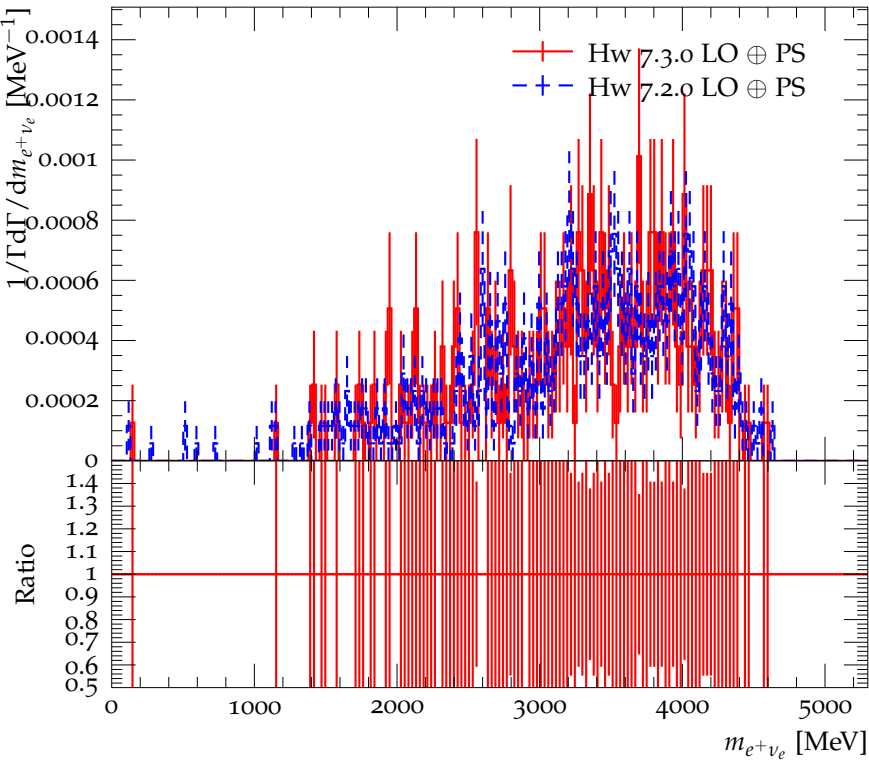
Mass of e^+v_e in the decay B^+ \rightarrow \rho^0 e^+ v_e
