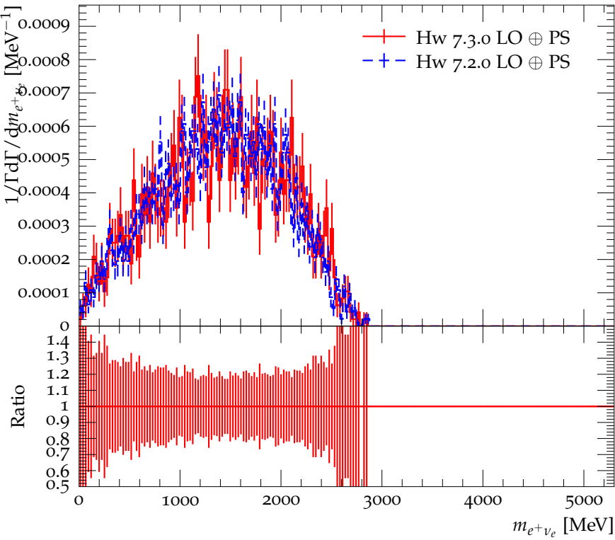
Mass of e^+\nu_e in the decay B^+ \rightarrow \bar{D}_1(2430)^0 e^+\nu_e
